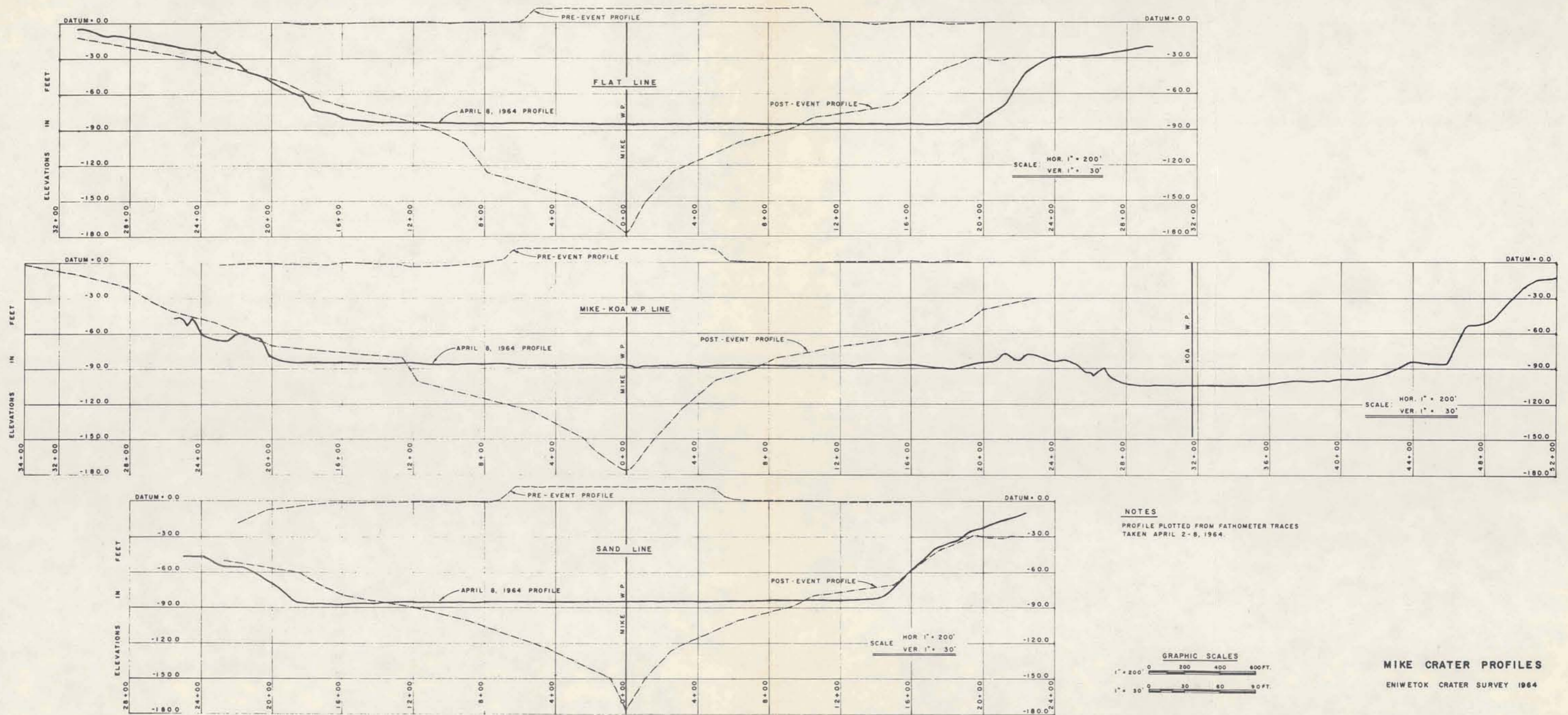
Fig. 7. Preshot, postshot, and 1964 survey profiles of Mike crater. Note the profile through the Mike and Koa zero points.
